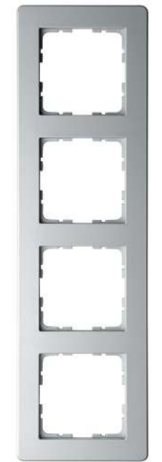
G1104S 4-gang W 86mm H 299mm D 9mm
